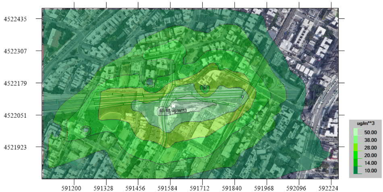
Figure 10 – 24-Hour PM 10 Scenario B Contours (µg/m 3 ), Cross Bronx at Macombs
