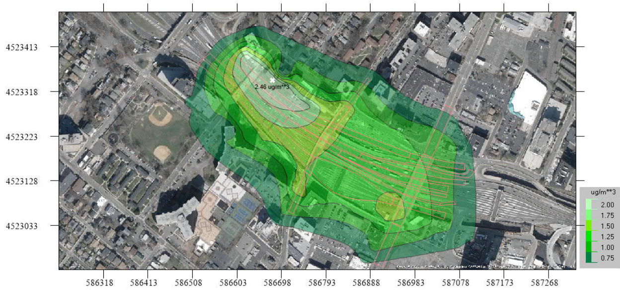
Figure 8 – AERMOD Model Screenshot, Cross Bronx at Macombs
