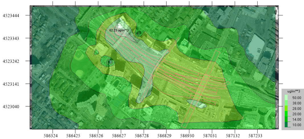
Figure 2 – 24-Hour PM 10 No Build Contours (µg/m 3 ), I-95 west of GWB
