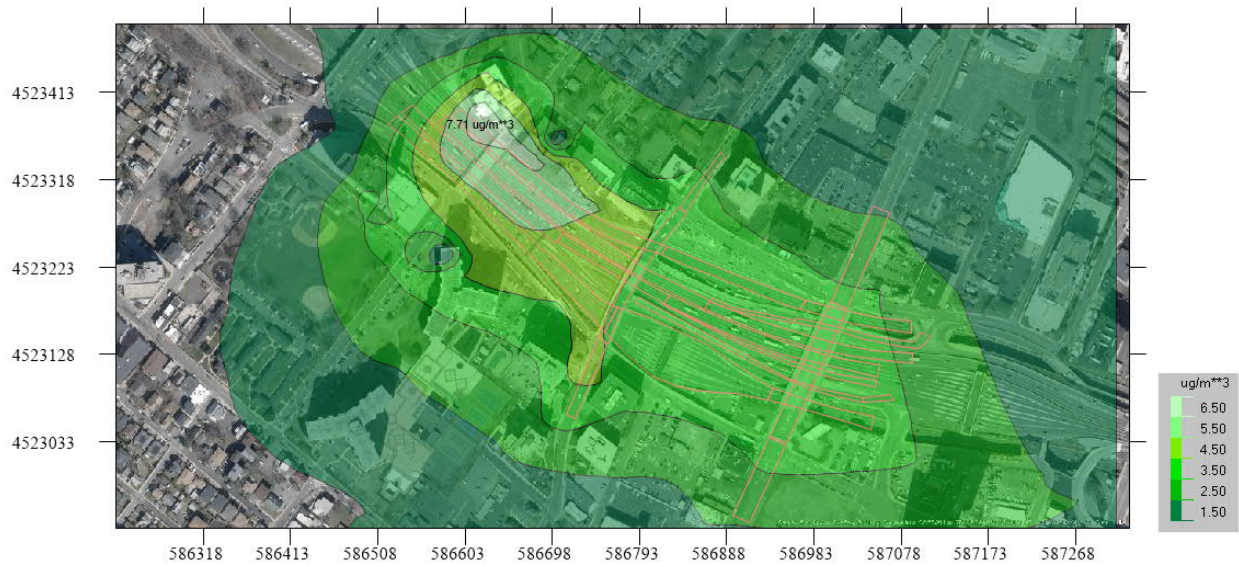
Figure 6 – Annual PM 2.5 No Build Contours (µg/m 3 ), I-95 west of GWB
