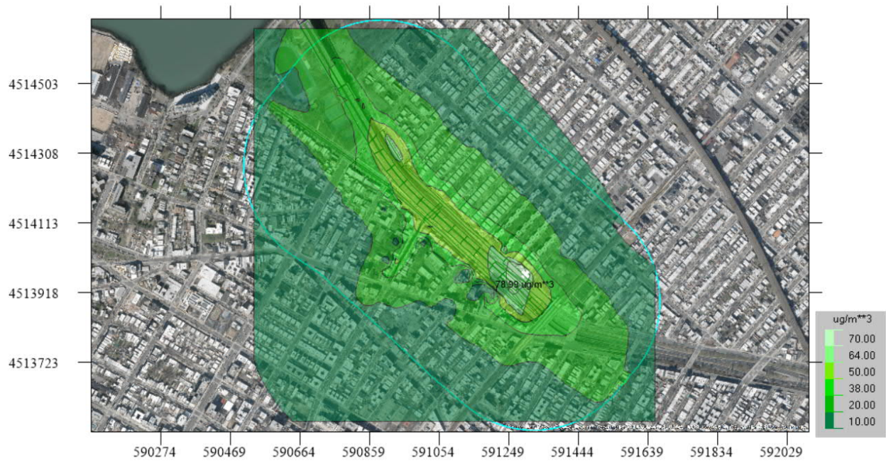
Figure 17 – 24-Hour PM 10 Scenario E Contours (µg/m 3 ), RFK Queens Approach
