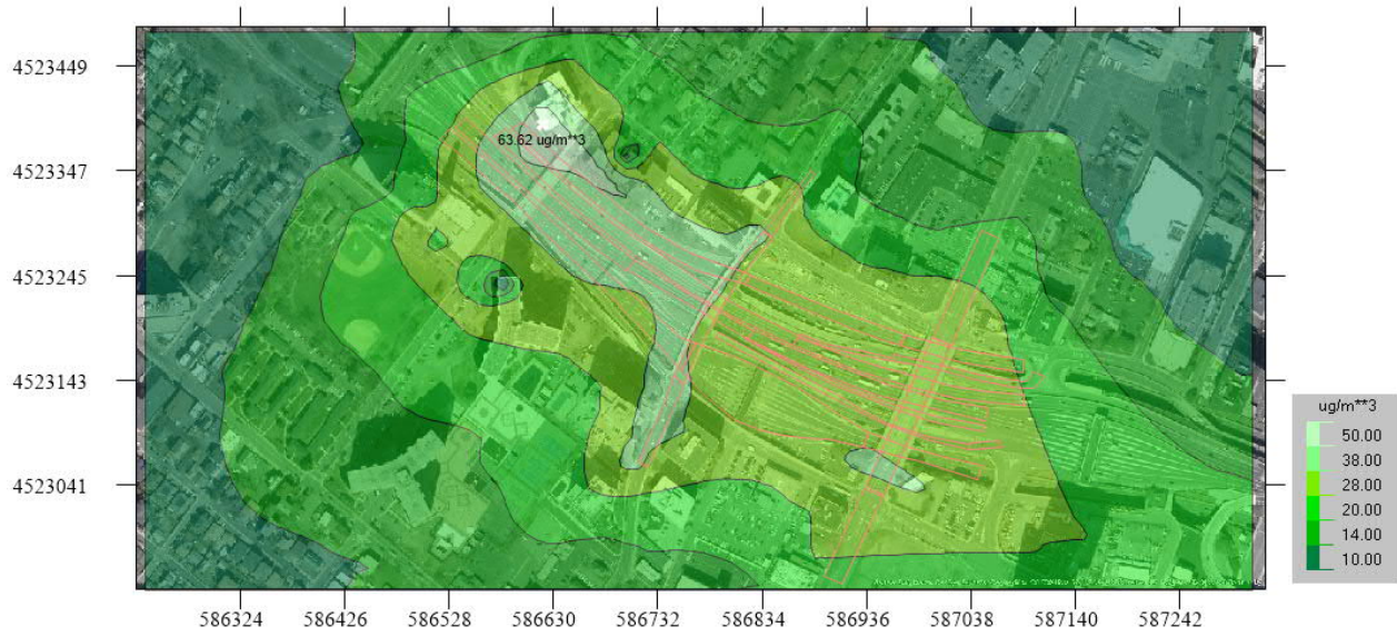
Figure 4 – 24-Hour PM 2.5 No Build Contours (µg/m 3 ), I-95 west of GWB
