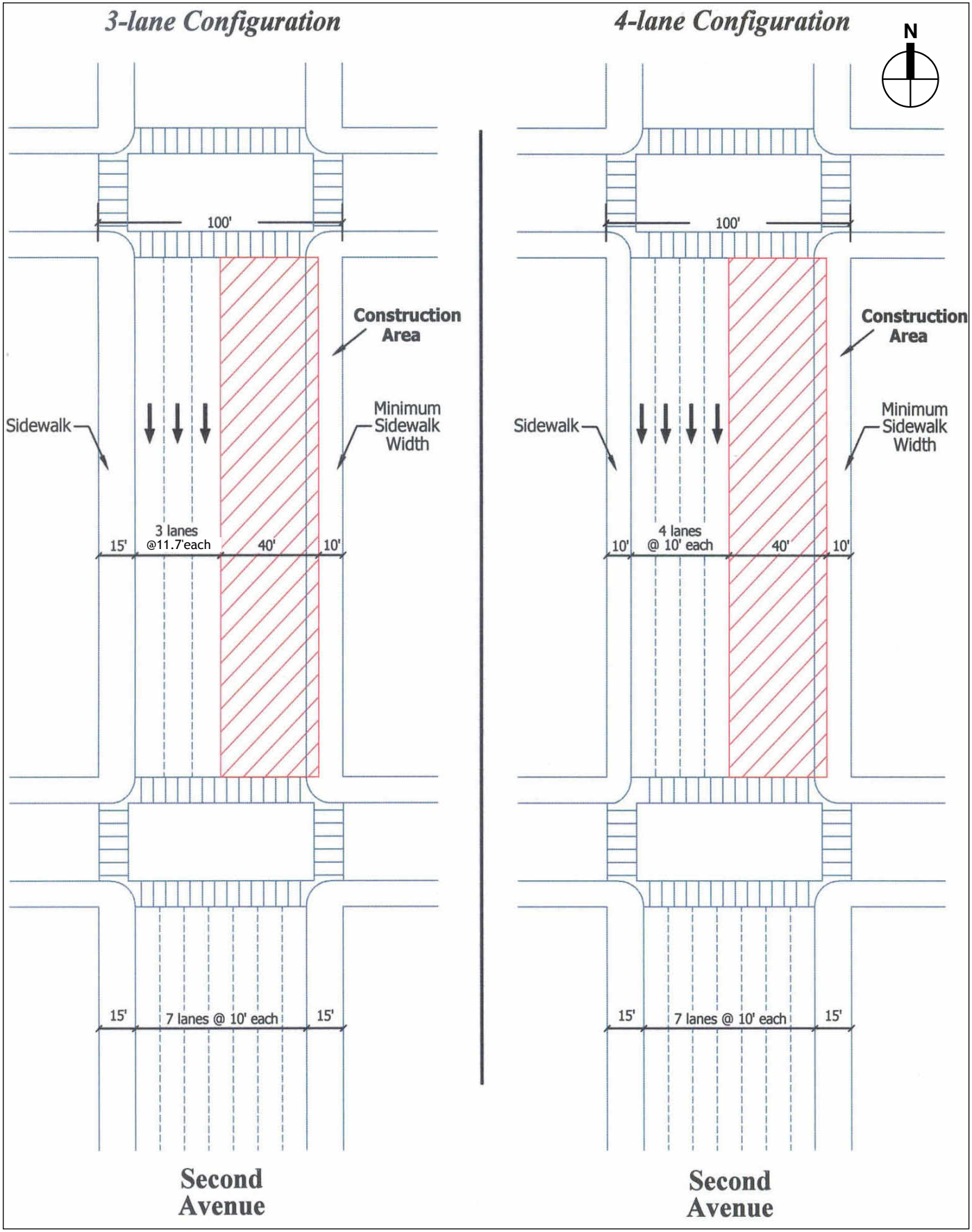
Figure 5D-3 Roadway Configuration Options During the Tunnel Construction Phase
